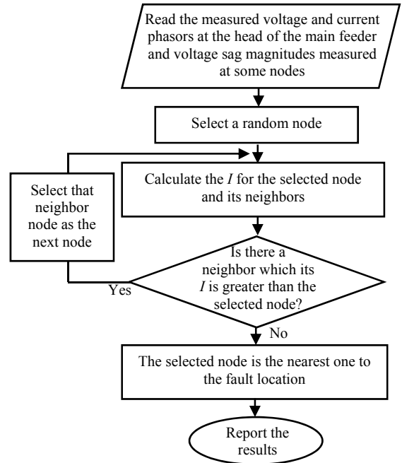
Fig. 4. Flowchart of the proposed fault location algorithm
