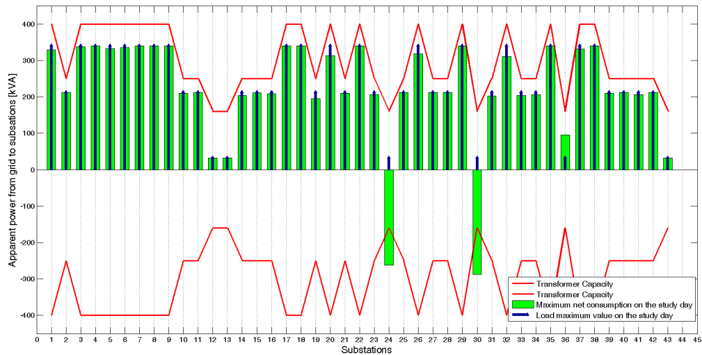
Fig. 8. Network results
