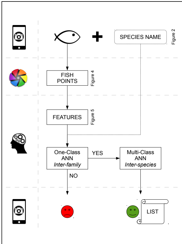
Figure 6. Classification Pipeline
