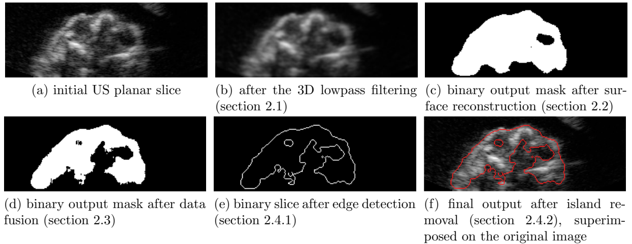
Figure 10: Example of successful application of the algorithm.
