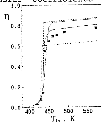
Fig. 7. Benzene conversion ( C_{\text{in}}=1000 ppmV; v_s=134,000 h ^{-1} ). Comparison of experimental results ( \blacksquare ) and model predictions using the mass transfer coefficient proposed by Hawthorn [13] (---), Votruba [14] (···) and Asako [15] [local (—) and average (---)].
