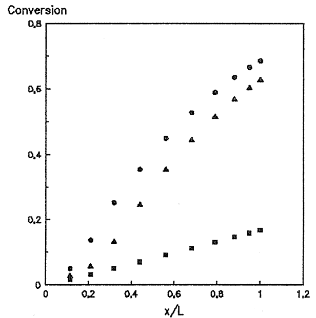
Fig. 9 - calculated (A) gas phase conversion vs reactor length in dynamic regime, C_0=1000 ppm G=10.6 l/min and Tin gas =170^\circ\text{C} .
