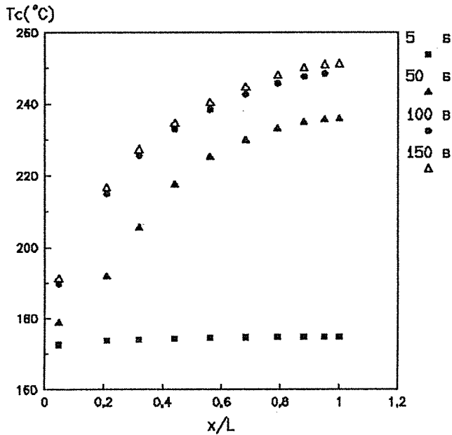
Fig. 8 - Calculated (A) catalyst temperature vs reactor length in dynamic regime, C_0=1000 ppm G=10.6 l/min and Tin gas =170^\circ\text{C} .
