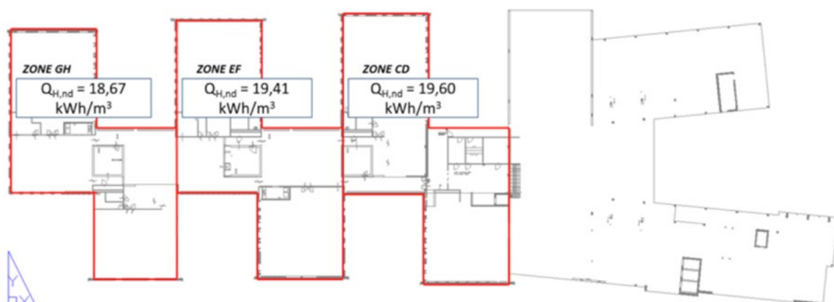
Figure 6. Building plan of the Zaanstad Town Hall with the indication of the building zones and their energy rating.
