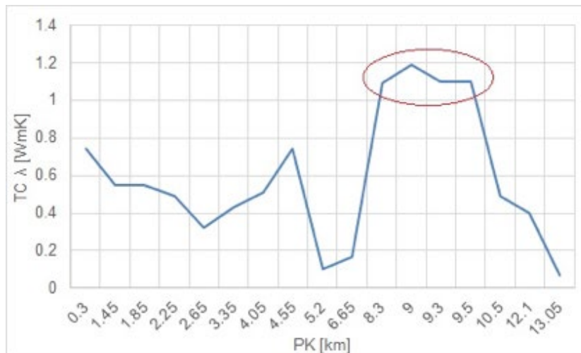
Figure 3. Thermal conductivity versus chainage.
