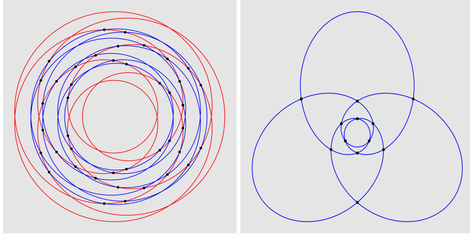
FIGURE 12. The link diagram of (K_{3,7}, K_{3,7}^*) (on the left) and the writhe diagram of K_{3,5} (on the right).
