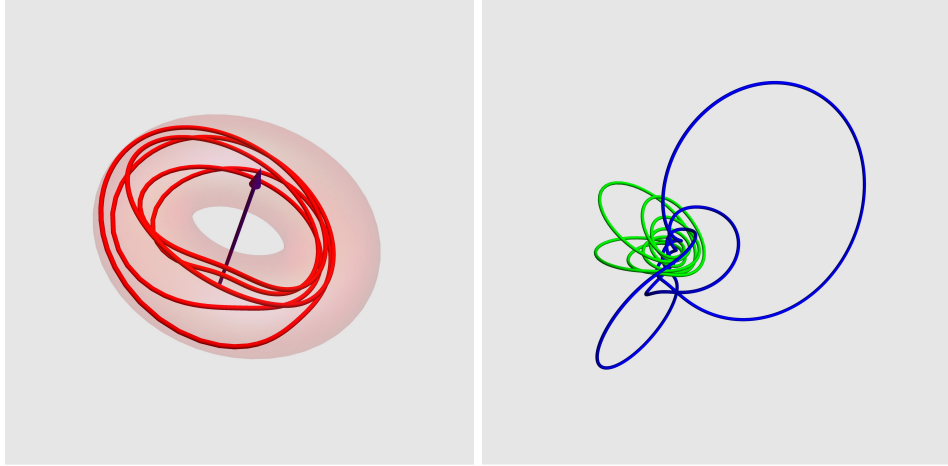
FIGURE 13. A closed homogenoeus curve with b = 2/5 trapped in the adS chamber (on the left) and the stereographic projections of its directrices from the point (1, 0, 0, 0) .
