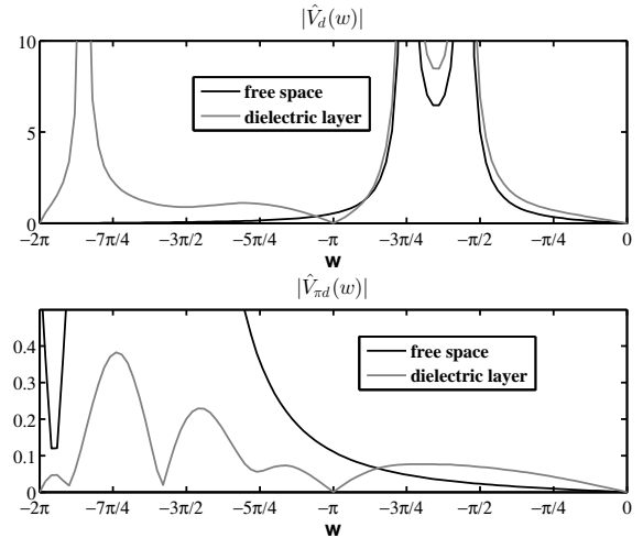
Fig. 9. Test case 2.1: the absolute value of the approximated spectra \hat{V}_d(w) and \hat{V}_{\pi d}(w) are reported for -2\pi \leq w \leq 0 respectively on top and on bottom of the figure.
