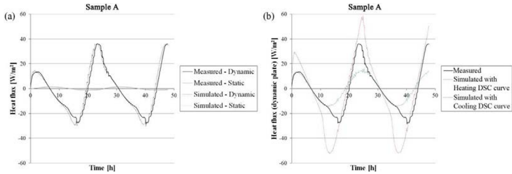
Fig. 1. Measured vs simulated heat fluxes for Sample A with: (a) data from inverse problem estimation; (b) data from DSC measurements.
