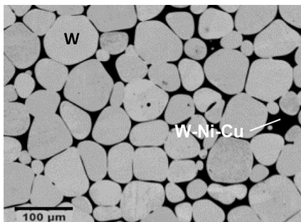
Figure 1. IT180 microstructure.
