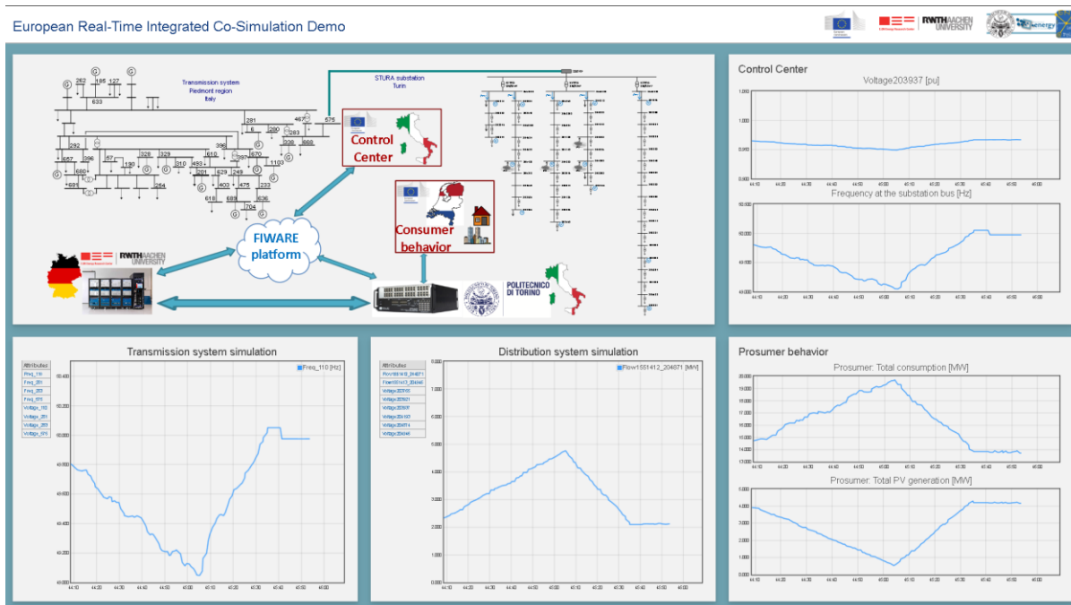
Figure 27 Demonstration final graphical interface - Technical layout
