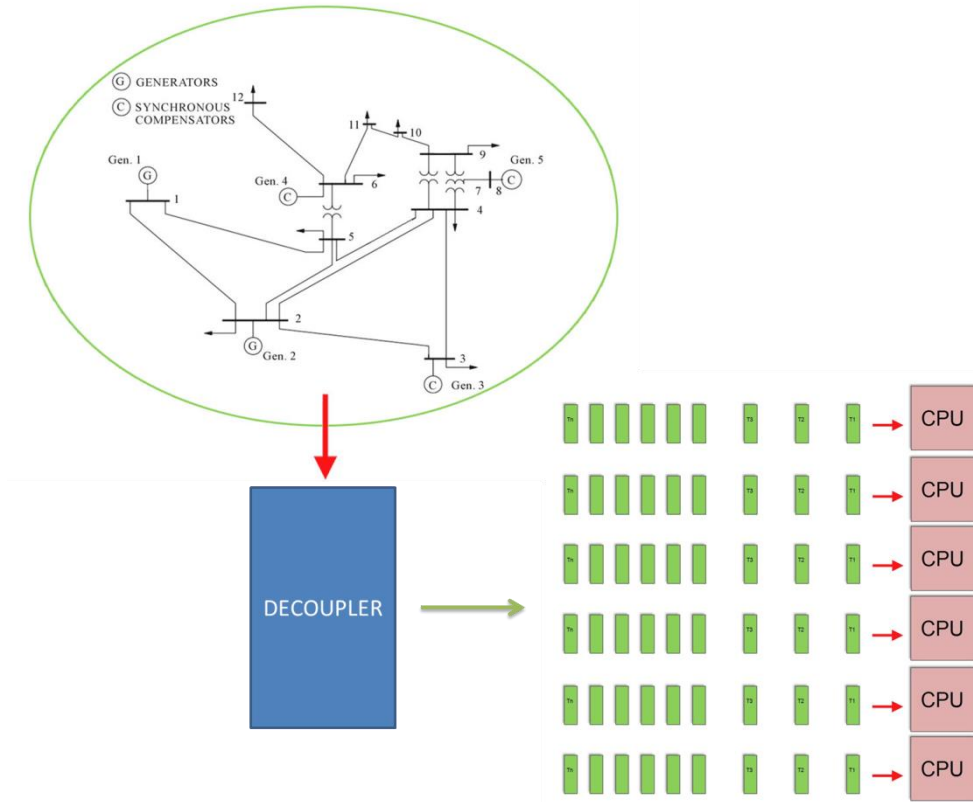
Figure 3 Parallel Computing
