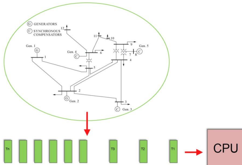
Figure 2 sequential computing
