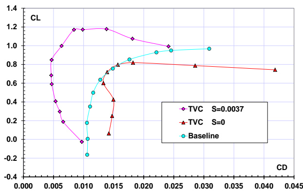
Fig. 9 - Drag polar comparison.
