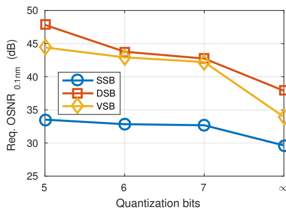
Fig. 12. Required OSNR (over 0.1 nm) to obtain \text{BER} = 10^{-3} for SSB (blue circles), DSB (red squares) and VSB (yellow diamonds), with different number of DAC quantization bits, at 80 km SSMF.
