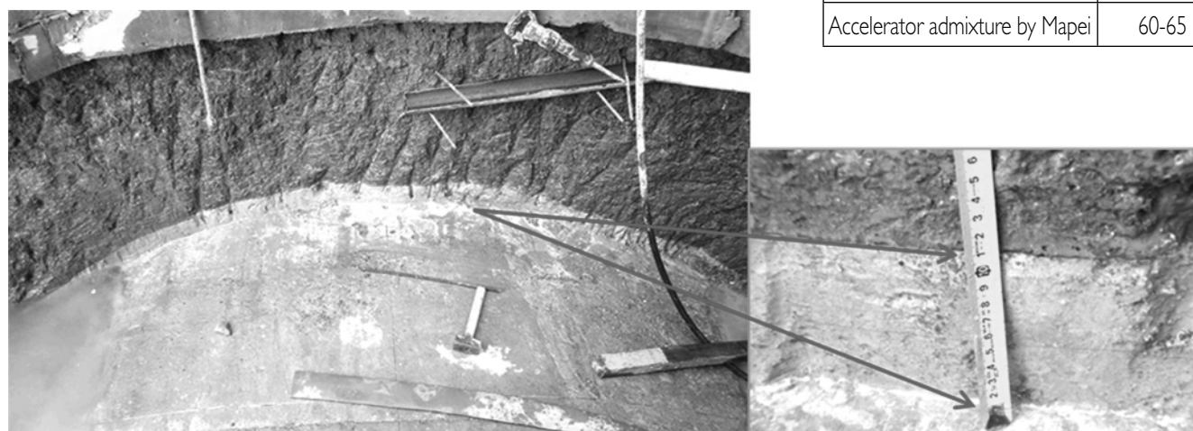
Fig. 6. View of the hardened grout excavated in a portion of the tunnel of Maldonado above the water table. It is possible to observe how the mix fills completely the void annulus (photos Mapei's archive).
