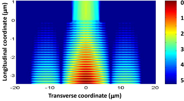
Fig. 2. Major component ( E_x ) field intensity (in logarithmic scale) in the (x, z) plane for the unprocessed VCSEL. z = 0 corresponds to the contact metal section; field is displayed starting from the quantum well region.
