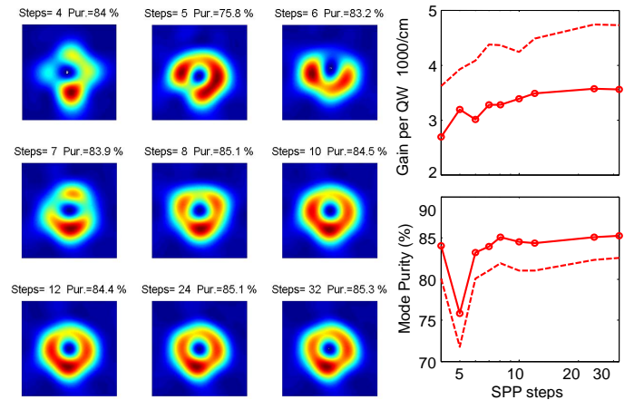
Fig. 7. Effect of SPP step number on the mode purity ( \ell = 1 ). Left: far-field intensity maps; mode purity and number of steps are given in the map titles. Right: threshold gains and mode purity vs. number of steps. The continuous curves refer to the lasing mode E_x , the dashed ones to the suppressed polarization mode.
