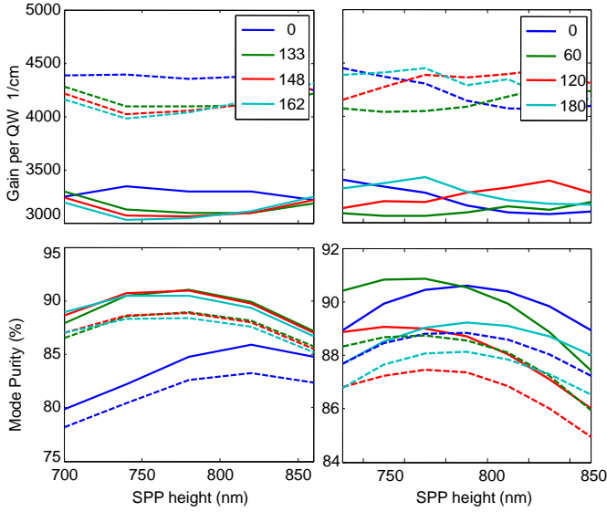
Fig. 12. Effect of introducing an ARC (refractive index 1.45) on the \ell = 1 SPP-VCSEL mode vs. the SPP height. Left: the curves refer to various ARC thicknesses (nm); the SPP base thickness is assumed to be 50nm. Right: the curves refer to various base thicknesses in the case of the optimal 148nm ARC.
