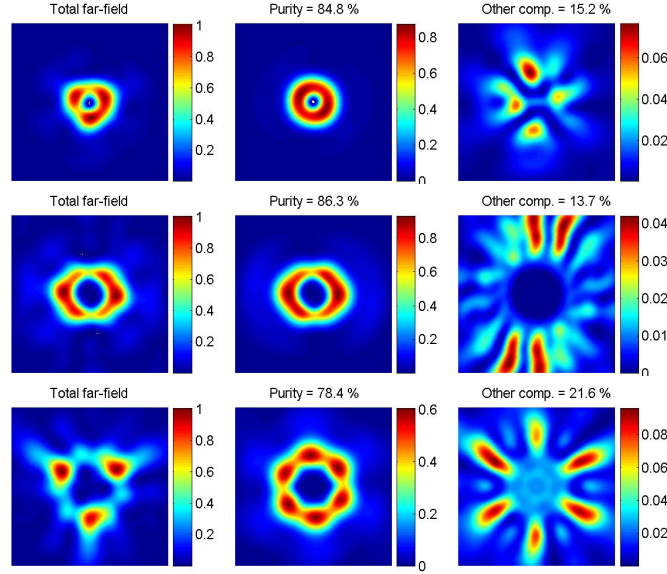
Fig. 6. Far-field patterns on 30 \times 30 degree window; rows refer to \ell = 1 to 3 SPPs, columns to different modal contributions: total fields, desired components, spurious components are reported in columns 1 to 3 respectively. The mode purity is given at the top.
