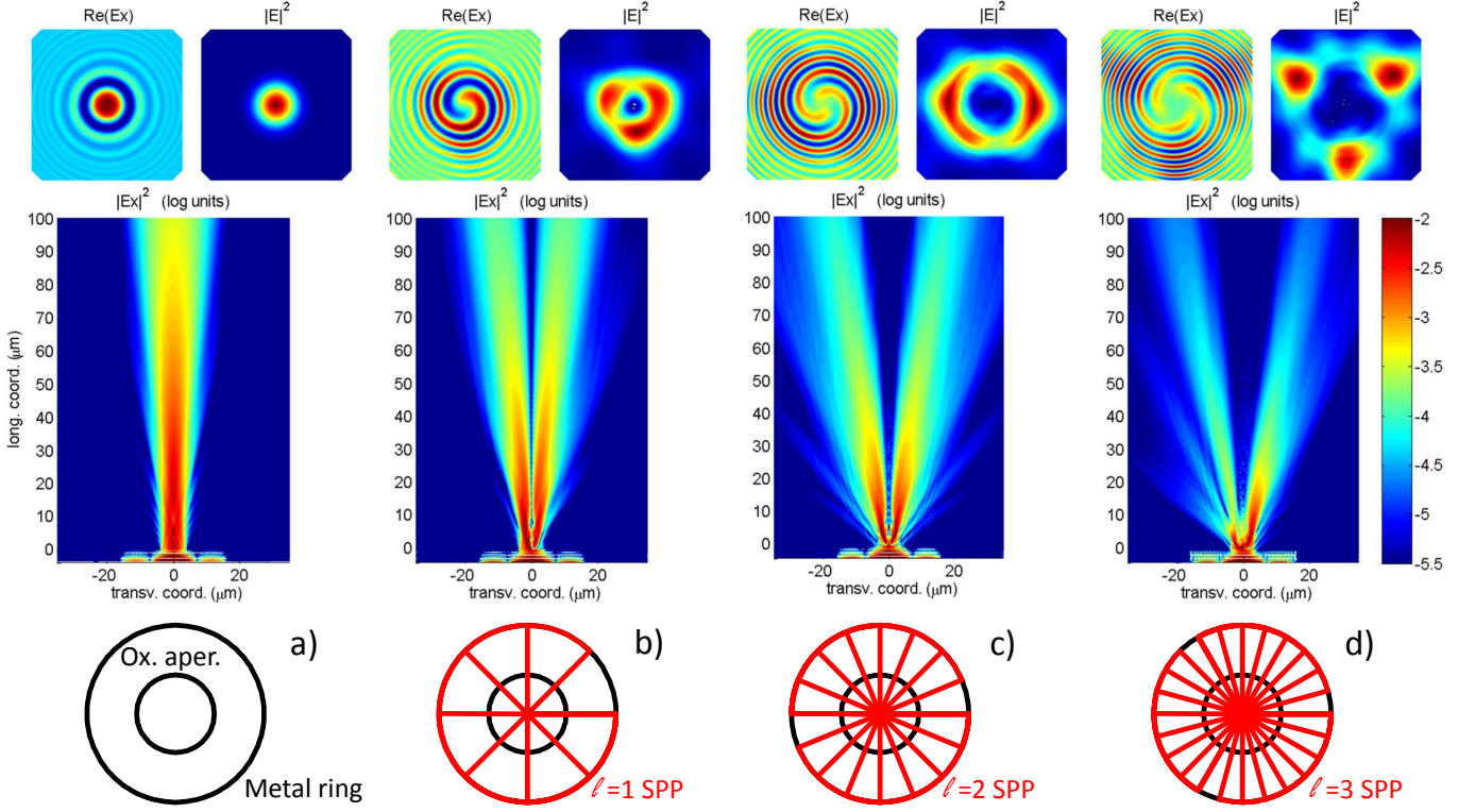
Fig. 4. Modal profiles of 4 devices: a , bare device, b – d , SPP with \ell = 1 to 3. Top maps refer to a 30 \times 30 \mu m^2 area at 100 \mu m distance from the outcoupling section. Center, (x, z) cuts of the field intensity. Bottom, top view of the transverse geometries; the SPP is shown in red.
