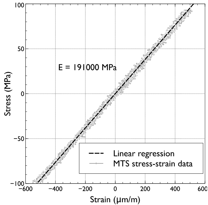
Figure 8: Experimental determination of Young's modulus: stress and strain measured in cyclic axial loading tests on a 30 mm \times 5 mm steel bar.
