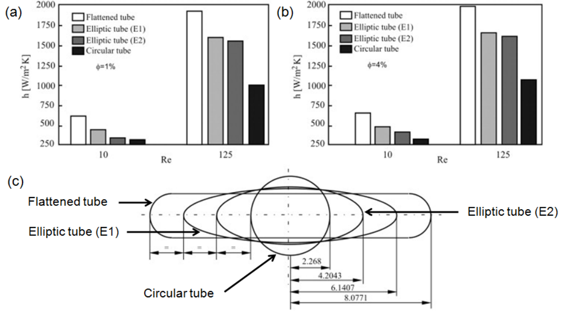
Figure 9: Heat transfer coefficient of a radiator tube. (a) Influence of Re and tube cross section on h_{nrf} at \phi = 1\% (b) Influence of Re and tube cross section on h_{nrf} at \phi = 4\% (c) Considered tube cross sections. Figure adopted from reference [255].
