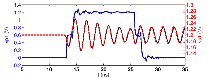
Fig. 4. Output port voltage response v_{p1}(t) and corresponding power supply fluctuation v_{s1}(t) for driver \mathcal{D}_B . Solid line: reference; dashed line: model.
