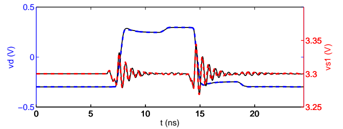
Fig. 3. Output differential voltage v_d(t) = v_1(t) - v_2(t) and corresponding power supply fluctuation v_{s1}(t) for driver \mathcal{D}_A . Solid line: reference; dashed line: model.
