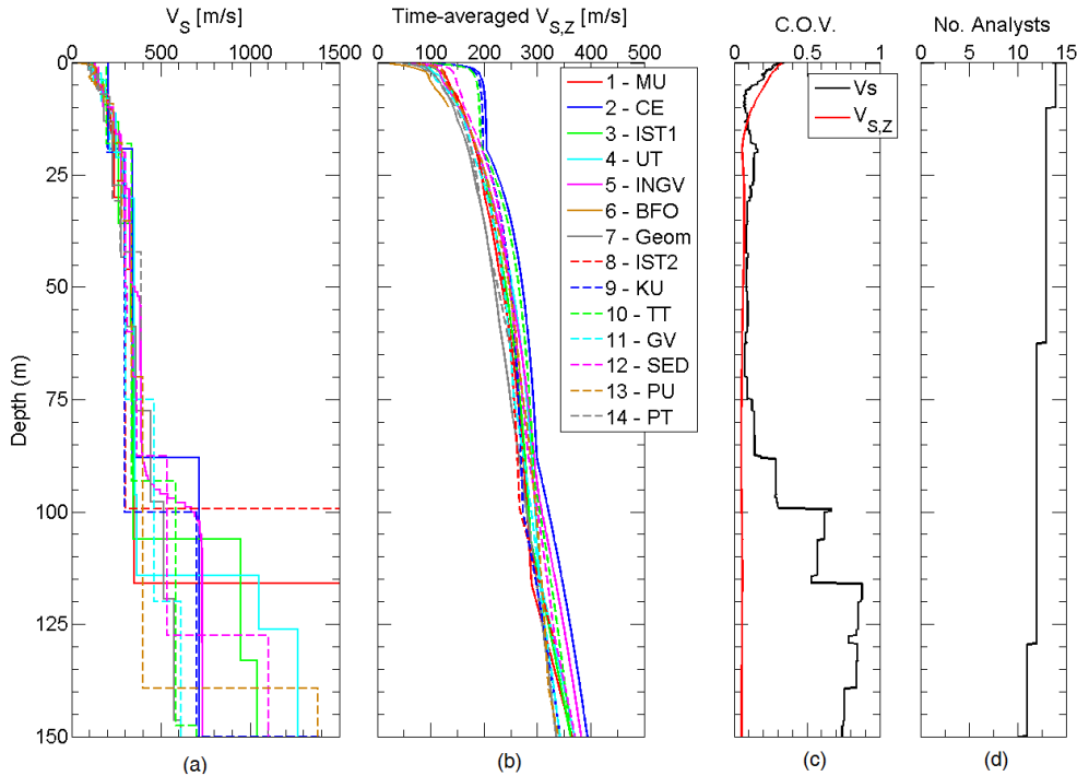
Figure 6 – Mirandola: close-up view of the top 150 m of Figure 5.
