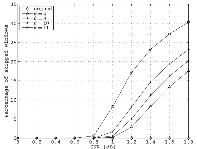
Fig. 3 Percentage of saved windows of the proposed window skipping technique for different values of \theta .
