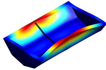
(b) Mode-2: 91.137 Hz
