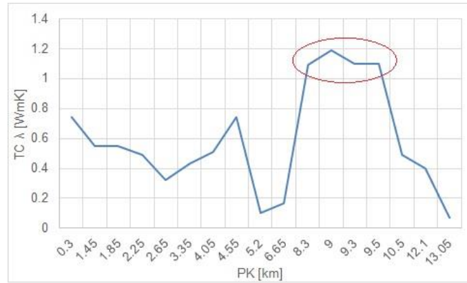
Figure 3. Thermal conductivity versus chainage.
