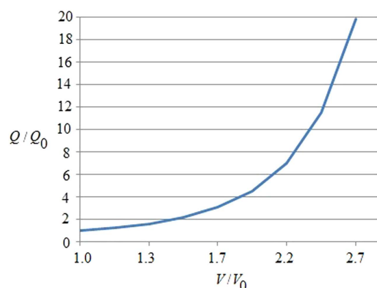
Figure 2. This figure represents the ratio of energy consumption vs. the volumetric growth of cancer. The y-axis is the ratio between the energy used by a cancer cell, Q , related to the energy used by a normal, non-cancerous cell, Q_0 . The x-axis is the ratio between the volume of cancer V related to its initial value V_0 at time 0. This result has been obtained by using Eq. (29). Note that a cancer cell and therefore tumor tissue consumes much more energy than normal tissue; moreover, the energy required by the cancer is proportional to the exponential tumor growth rate.
