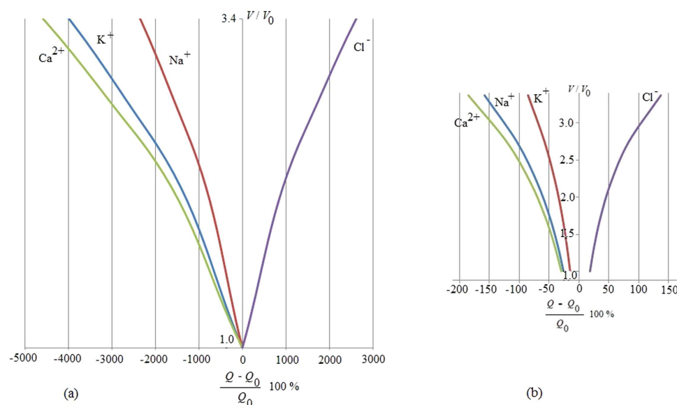
Figure 3. The figure represents the volumetric growth of cancer tissue under a magnetic field (50 \mu T, 40 Hz) in relation to the energy used by the cancer with regards to the ion involved. The y-axis represents growth, i.e. the ratio between the volume of cancer V related to its initial value V_0 . The x-axis displays the ratio (in percentage) in energy consumption used for growth between a cancer cell and a normal, non-cancerous cell; here, Q is the energy used by the cancer cell while Q_0 is the energy consumed by the normal cell; minus (–) and plus (+) are related to the motion of the ions in relation to the membrane's bioelectric field; consequently, in the case of \text{Cl}^- inflow the cell gains energy, which in turn can be used for continued growth, while, to process \text{Ca}^{2+} , \text{K}^+ and \text{Na}^+ inflow, the cell loses energy and thus growth potential as it works against the membrane potential to sustain the influx of these ions. As the tumor grows, all ion fluxes change but their percentage changes are much larger when the tumor is exposed to the magnetic field in (a), reflecting a much more pronounced consumption of ATP to process these fluxes. The inhibitory effect of the magnetic field is evident as the tumor, to achieve the same volumetric growth, is forced to consume much more energy in (a) than in (b) when it is not exposed to a magnetic field. Still, since \text{Cl}^- influx increases also in (a), particularly at later growth stages, this further supports the argument that magnetic field therapy may lose efficacy eventually (which is being explored in more detail in Fig. 4).
