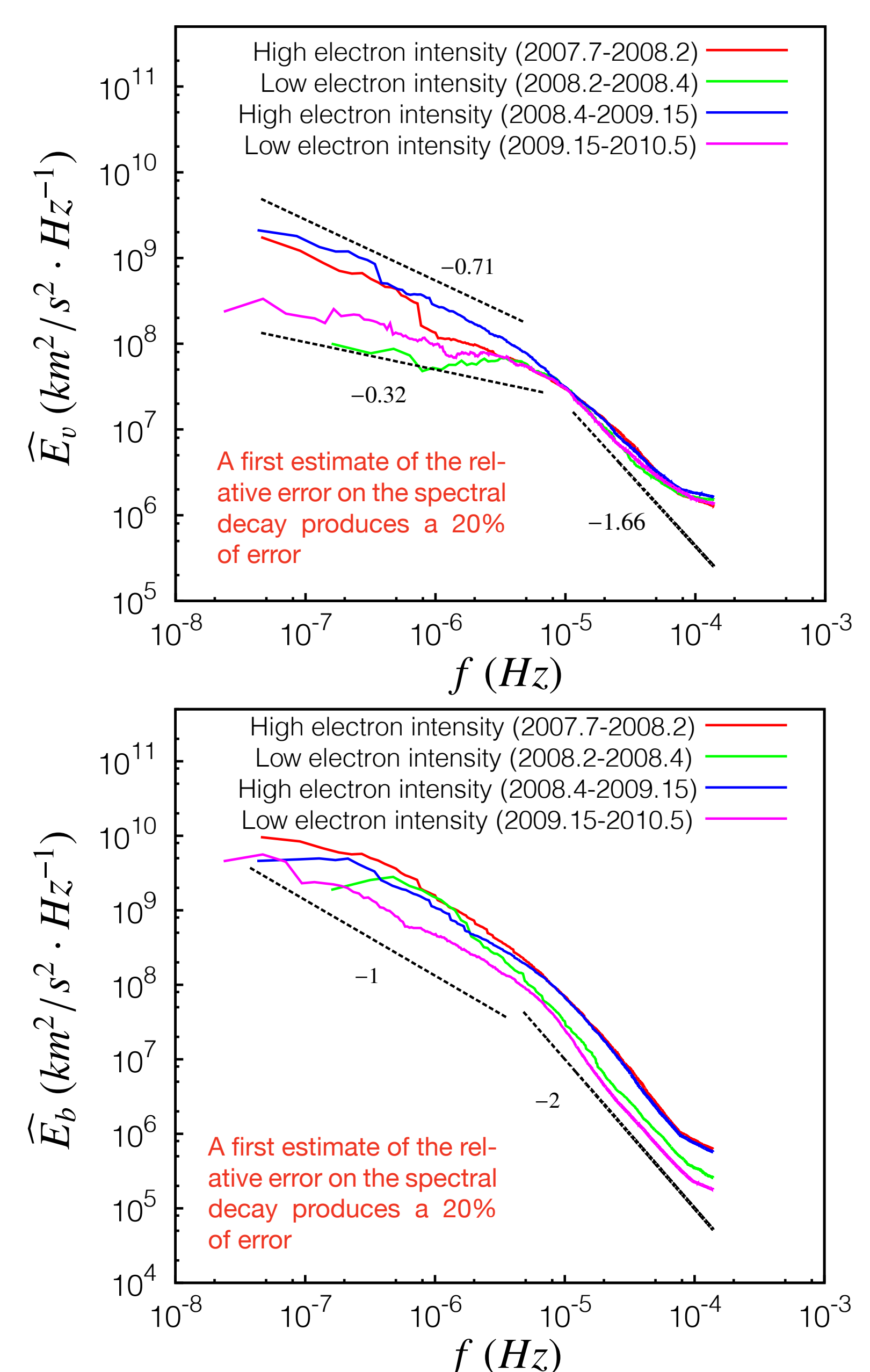
FIG. 4. Preliminary power spectra of plasma velocity (top) and magnetic field (bottom) in the heliosheath. Four subranges are selected by considering the periods when V2 was in the sectored (high electron intensity) or in the unipolar (low electron intensity) regions (see figures below and [7, 8]). Spectra are computed by using the correlation method described in the bottom of the poster and by considering hourly averaged data.
