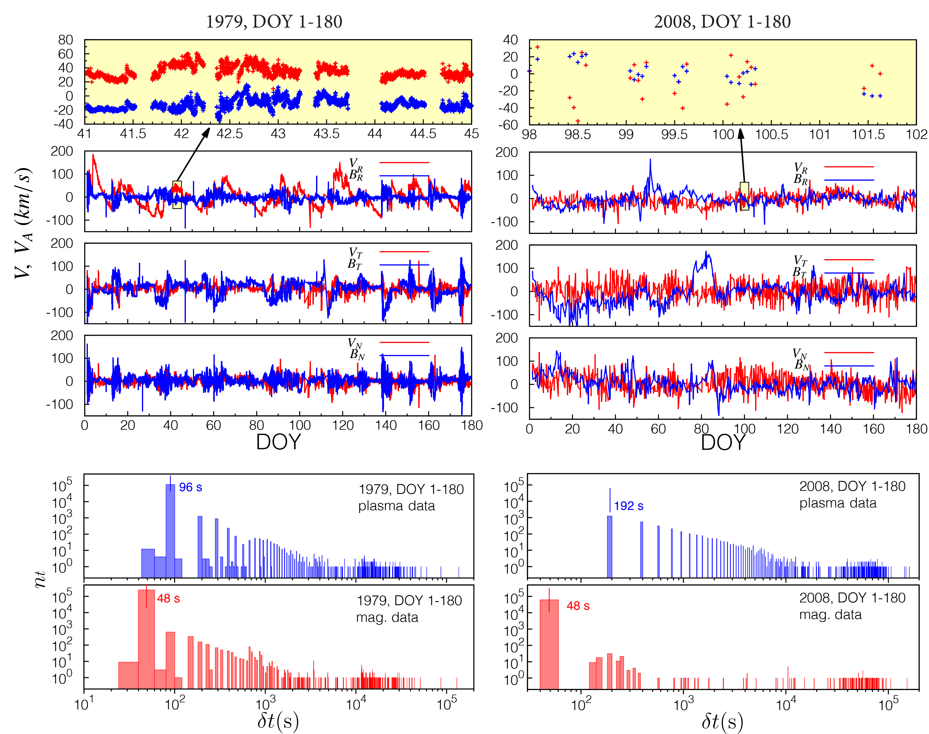
FIG. 1. Datasets. Upper panels: instantaneous values of plasma velocity (red lines) and magnetic fields (blue lines) recorded by Voyager 2 in the first 180 days of 1979 (left) and 2008 (right). The RTN Heliographic reference frame is used. The magnetic field is represented using the Alfvén units to make uniform the physical dimensions. In the two top panels, the magnification of 4 days periods make the data gaps apparent. Datasets from Voyager 2 are lacunous and irregularly distributed. In order to perform spectral analysis, methods for signal reconstruction of missing data should be implemented, see the poster bottom. Lower panels: gap distributions are shown. Missing data are about 30% in 1979 and 75% in the Heliosheath (2007.7-2010.5).
