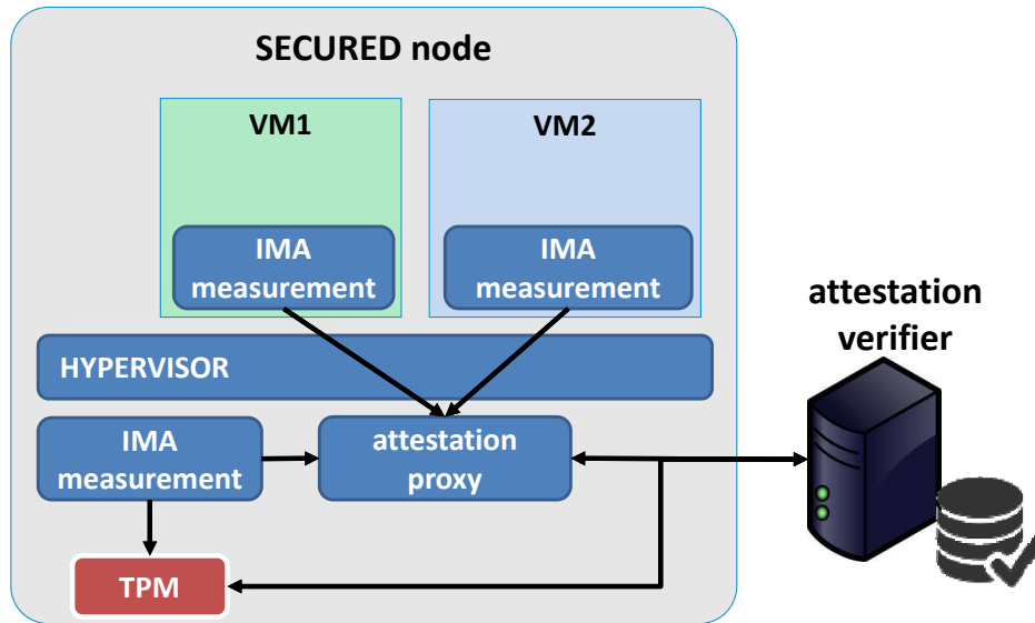
Fig. 7. IMA-based attestation architecture.
