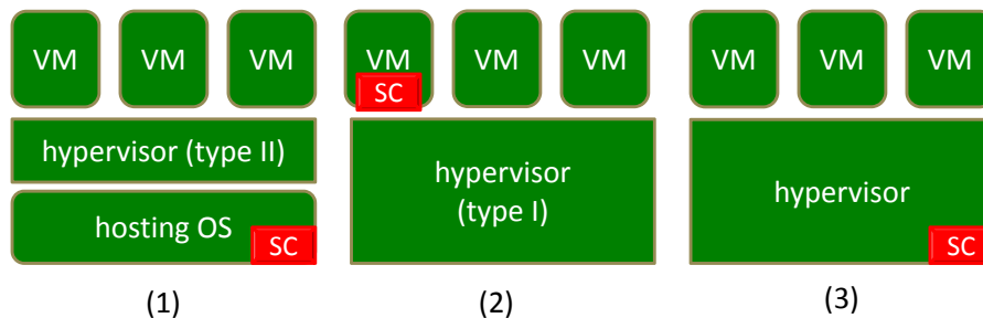
Fig. 6. Possible placement of the attestation supporting component.
