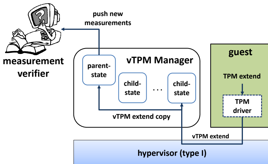
Fig. 5. Solution architecture in [11].
