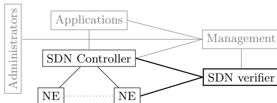
Fig. 2. Logical overview of the proposed monitoring architecture
