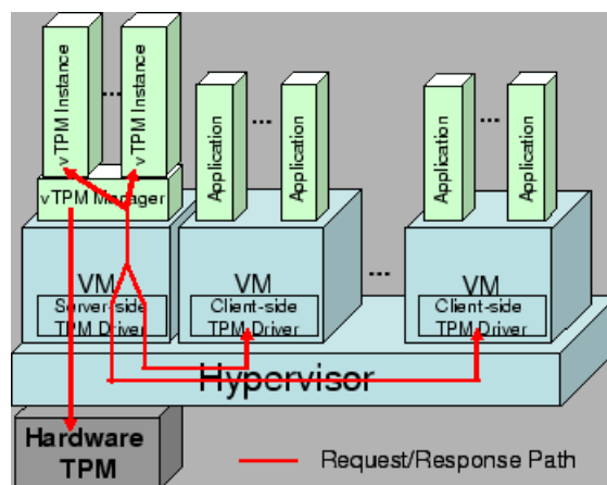
Fig. 4. The vTPM architecture [10].
