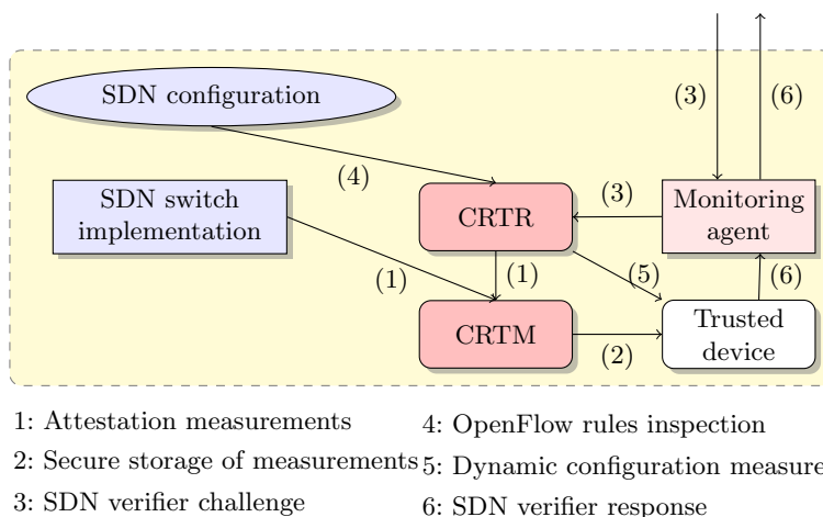
Fig. 3. Network element component architecture target
