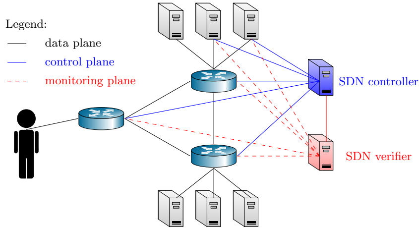
Fig. 1. A typical SDN topology, enhanced with a SDN verifier.
