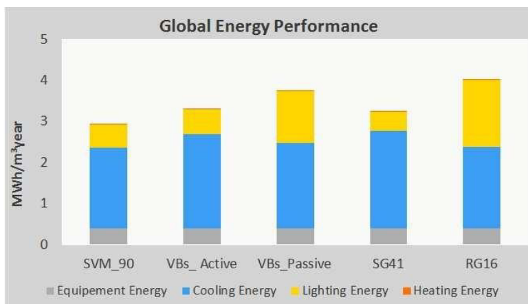
Fig. 3. EP_b , EP_c , EP_1 and EP_{gl} values found in step 2. The SVM shows the best performance, minimizing the building global energy consumption (up to -27% compared to RG16). This is mainly due to the reduced energy demand for lighting (up to -65.7% compared to RG16) and, to a lower extent, for cooling (up to -17.2% compared to SG41).
