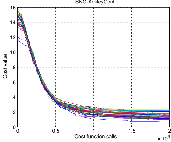
Figure 4. Best agent behavior over 50 trials, considering N_{pop} = 500 .
