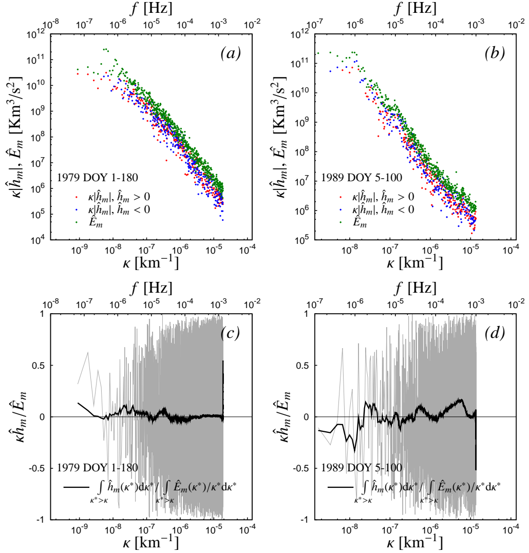
Figure 5: (a,b) Wave numbers spectra of the magnetic helicity density and of the magnetic energy \langle b'_j b'_j \rangle / 2 in Alfvén units. These spectra are obtained by means of the Taylor hypothesis, see section 3. The mean speed is that computed over the whole time interval, see Table 1. For graphic clarity, in panel (a), for frequencies above 10^{-6} Hz, not all the points of the spectra of the magnetic helicity are shown. The same in panel (b) above 10^{-5} Hz. (c,d) Relative normalized magnetic helicity \sigma_m(\kappa) = \kappa\hat{h}_m/E_m(\kappa) . The thick line indicates the cumulative relative helicity integrated from a given \kappa to the highest observed wavenumber.
