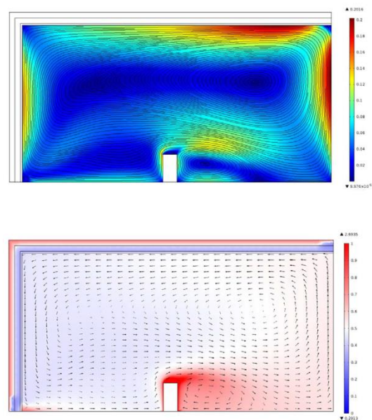
Figure 6 – The air velocity field calculated in steady-state conditions (above) and a snapshot of the relative humidity distribution in the air volume and within the envelope (below) for vents configuration n.1
