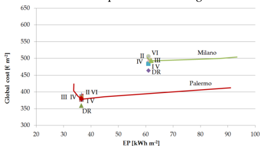
Fig. 2 – Residential Cost Optimal values for different economic scenarios
