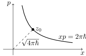
Fig. 4. The point z_0 minimizes the distance of the zero set \Theta(z) = 0 from 0.
