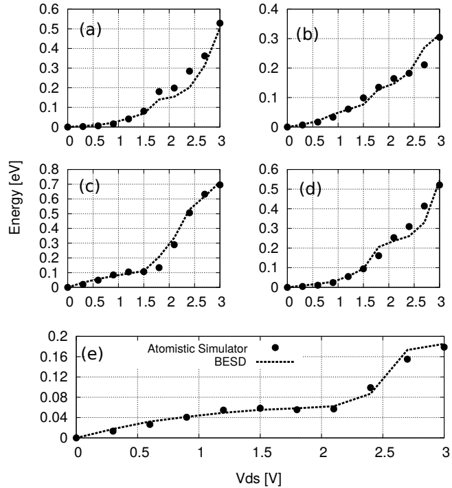
Fig. 9 Comparison of the area of the integral of the transmission spectrum covered by electrode chemical potential as a function of bias voltage of different molecules at zero gate voltage (a) OPV, (b) OPE, (c) 3TT, (d) 4TT and (e) 5TT. Dashed lines represents the proposed model results and the dots are related to atomistic simulation [45,48] results.
