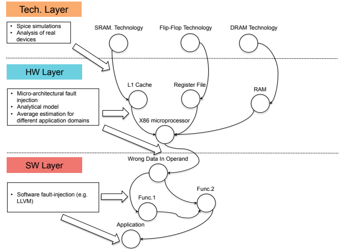
Figure 3: System level reliability evaluation using Bayesian a bayesian model of the system. Nodes of the model represent system resources (e.g., technology, hardware, software), while edges represent how these resources influence each other when faults arise in the system.
