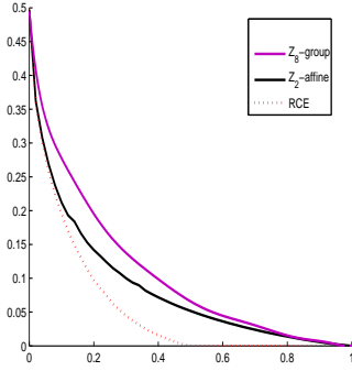
Fig. 2. A comparison of \delta_8(R) (purple line) and \bar{\delta}_\eta(R) where \eta: \mathbb{Z}_2^3 \rightarrow \mathcal{X} is the Gray labeling described in Fig.1. As a reference \delta_8(2R) (which is the typical normalized minimum distance of the RCE) is plotted in dotted red. For the specific choice of the binary labeling \eta: \mathbb{Z}_2^3 \rightarrow \mathcal{X} , and the chosen resolution, it seems that \bar{\delta}_\eta(R) = \underline{\delta}_\eta(R) .
