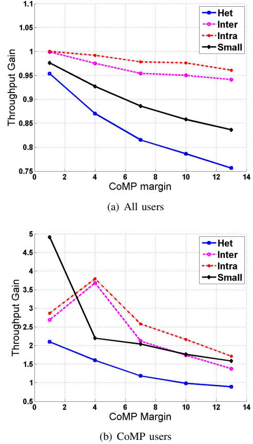
Fig. 2. Throughput Gain for all users (a) and for CoMP users (b) as a function of CoMP margin for different scenarios (M=15, S=50, CPP=30%).
