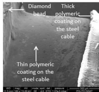
Figure 3: SEM image at low magnification of the junction between the diamond beads and the steel rope
