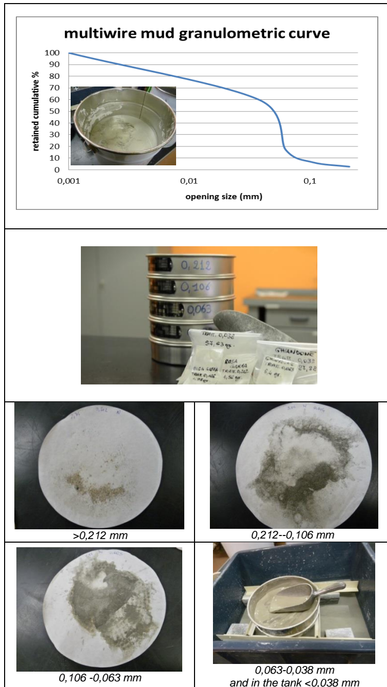
Figure 2: size distribution process and characterization of multiwire muds
