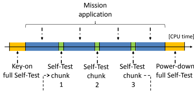
Fig 1: On-Line Self-Test application example.
