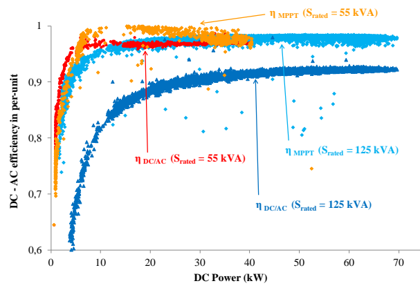
Fig. 18. MPPT and DC-AC efficiencies of GMPV and BIPV inverters.
