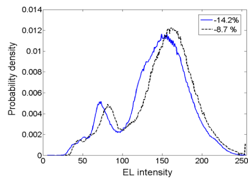
Fig. 15. Correlation between probability density function of the EL intensity signal and the module power loss.
