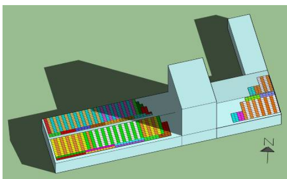
Fig. 3. Simulation of shadows on the closest PV strings (10:30 am in spring).
