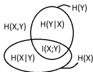
Figure 1: Venn diagram of mutual information I(X;Y) associated with correlated variables X and Y. The area contained by both circles is the joint entropy H(X,Y) . The lower circle is the individual entropy H(X) , such as the upper circle is that of H(Y) .
