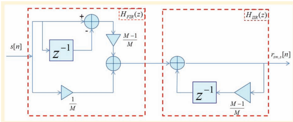
FIGURE 2 Block diagram of the carrier-smoothing system for the common component s[n]
