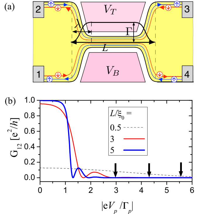
FIG. 1. (Color online) (a) Sketch of the extended tunnel junction setup, characterized by a total length L , where the amplitudes for spin-preserving and spin-flipping tunnel processes increase from 0 to the bulk values |\Gamma_p| and |\Gamma_f| , over a length scale \lambda . Two side gate voltages V_T and V_B are applied across the tunnel junction. (b) The transconductance |G_{12}| = (e^2/h)R_p is plotted as a function of the charge gate voltage V_p = (V_T + V_B)/2 , for three different ratios of the junction length L to the length scale \xi_0 = \hbar v_F/|\Gamma_p| , and for \lambda = 0.25L . While for short junctions the reflection is always small and weakly dependent on V_p , for extended junctions |G_{12}| drops from the quantum of resistance to 0, within an energy window around the bulk spin-preserving tunneling amplitude |\Gamma_p| . The vertical arrows indicate the regime where the condition R_p \simeq 0 for revealing the spin-flipping partition noise is fulfilled [see Fig. 2(b)].
