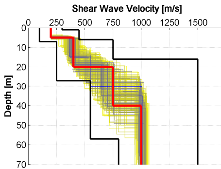
Figure 1: Monte Carlo inversion results: in red the true model and in colour scale the selected 200 models out of 10^5 simulations, the colourscale represents the misfit. The model space from which the random sampling is performed is indicated by black lines.
