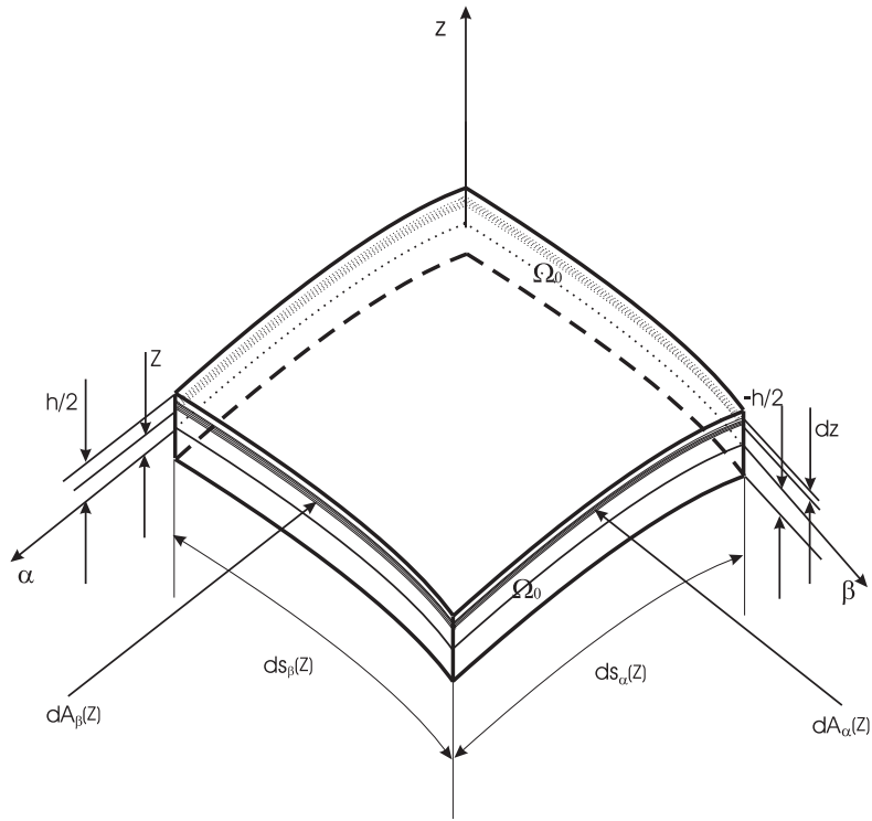
Figure 1: Geometry, notation and reference system for shells.
