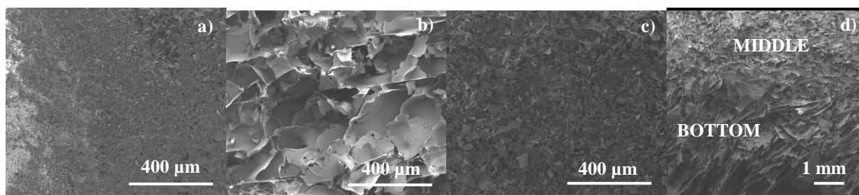
Figure 2: SEM images of a mannitol 5% samples in the case of (a) uncontrolled freezing and freezing induced at (b) -5^{\circ}\text{C} , (c) -10^{\circ}\text{C} , and (d) with high filling volume (5 ml with respect to 3 ml of the other samples).
