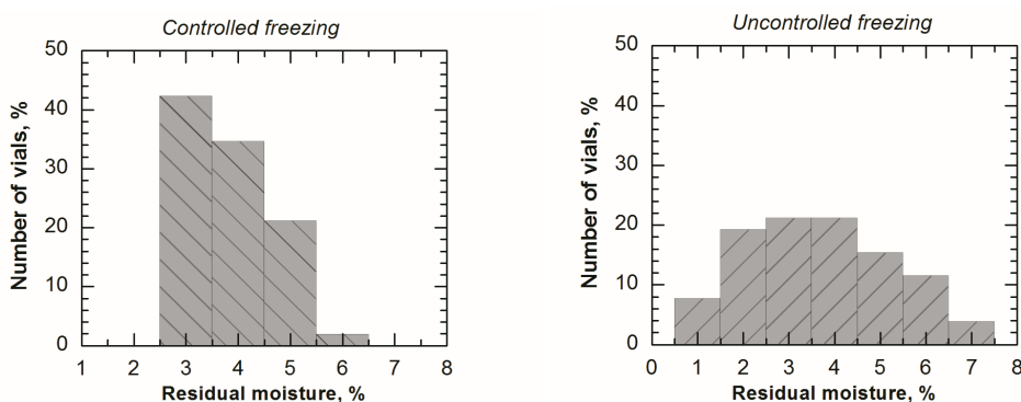
Figure 1: Distribution of moisture content at the end of the primary drying stage in the case of controlled and uncontrolled freezing.
