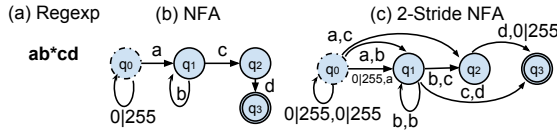
Fig. 1. A simple regular expression in its (a) “textual” representation, (b) NFA form and (c) 2-stride NFA form.
