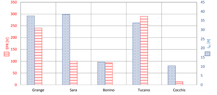
Fig. 10. EPR and earth currents in the considered substations.
