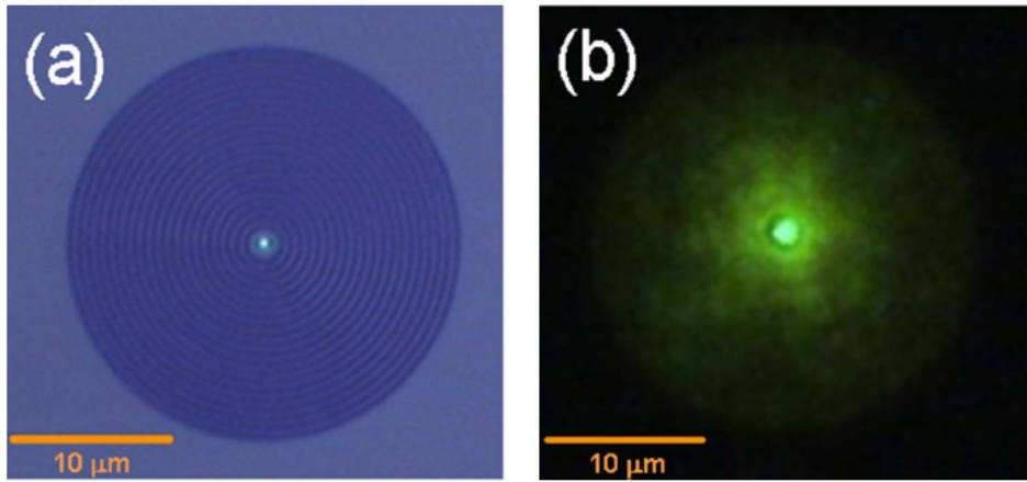
Figure 5.3: (a) Reflection bright-field image of a circular grating made through a top objective ( NA = 0.95 ) and laser focusing in the central spacer; (b) direct plane image of fluorescence collected by the NA = 1.49 objective
