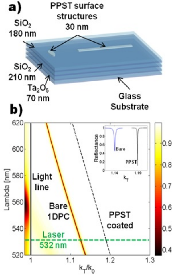
Figure 2.1: (a) 3D sketch of the polymeric refractive structures fabricated on top of the 1DPC. (b) Calculated TE reflectance map function of lambda and the effective index of the mode k_T/k_0 . To evaluate the dielectric loading effect, the position of the dip in reflectance for the multilayer coated with 30 nm of PPST is reported (black dashed line). An intensity profile extracted along the green dashed line (at \lambda = 532nm ) is reported in the inset.
