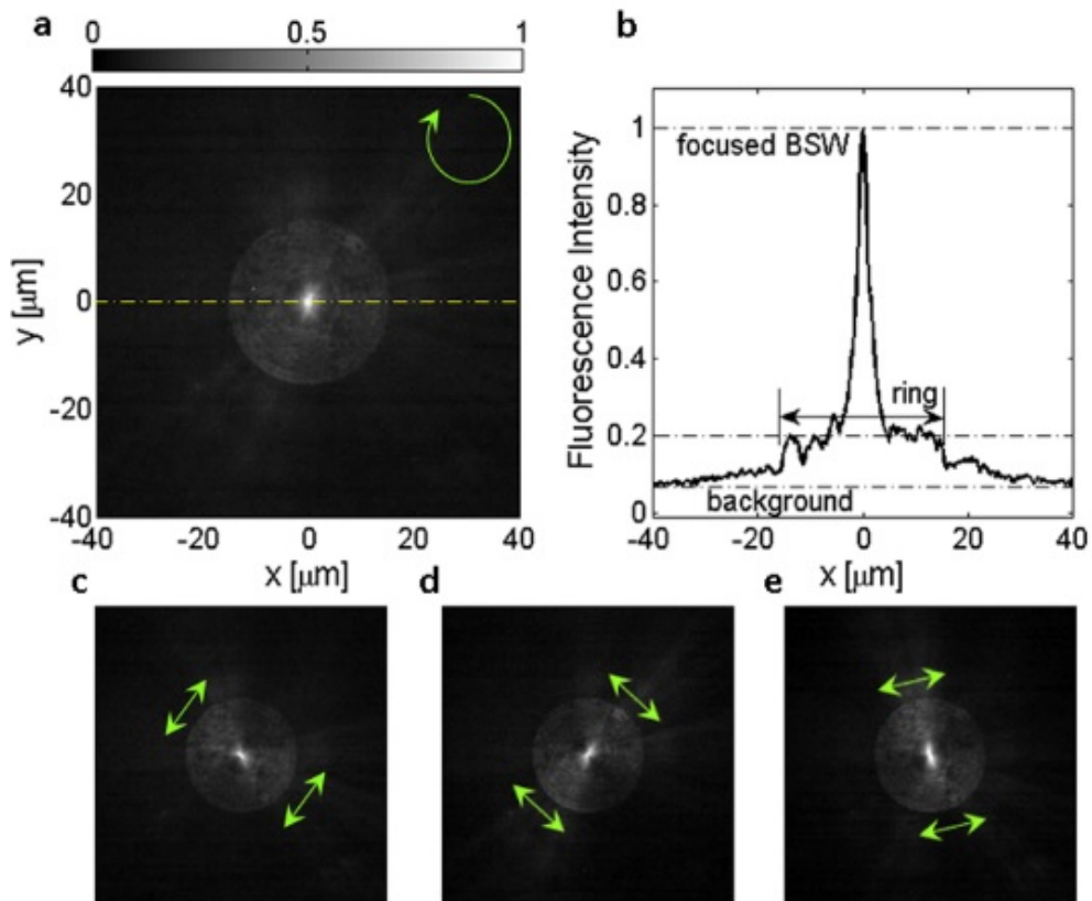
Figure 2.11: (a), fluorescence image of a laser BSW coupled and focused by a circular grating ( D = 8\mu m , L = 520nm ) on "low leakage" multilayer. Illumination is a collimated, circularly polarized laser beam. (b), cross-sectional fluorescence intensity along the dashed line in (a). (c), (d), (e), same as in (a) with an incident laser beam linearly polarized as sketched by the arrows in the figures. All images are collected by means of the setup sketched in 1.4.
