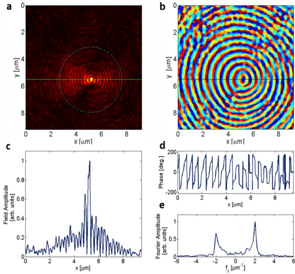
Figure 2.10: (a), amplitude and (b), phase distribution of the leakage radiation associated to a converging laser BSW. Coupling is performed by illuminating a circular grating ( D = 5\mu\text{m} , L = 520\text{nm} ) on a "regular" multilayer with a linearly polarized ( y -direction) laser ( \lambda = 532\text{nm} ). The dashed circle indicates the boundary on the inner spacer. (c), cross-sectional field amplitude profile along the horizontal line shown in (a). (d), cross-sectional field phase profile and (e) its corresponding Fourier spectrum amplitude along the horizontal line shown in (b).
