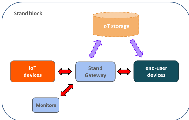
Fig. 2: Architecture design
