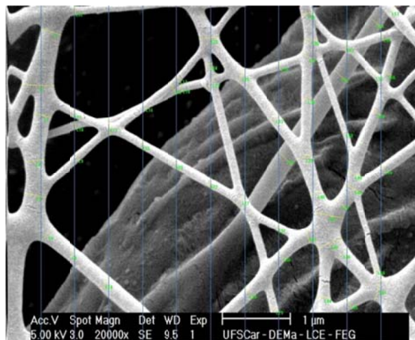
Fig. 2. 20000x image, showing nanofiber details.
