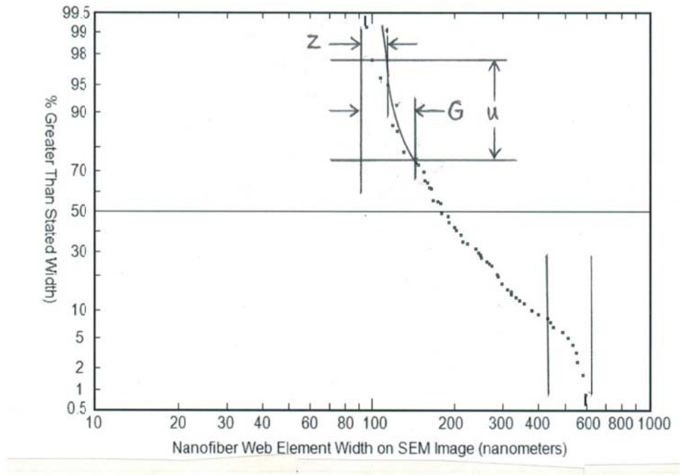
Fig.6 - Curve-fitting to truncated-log-normal distribution: tail asymptotes
